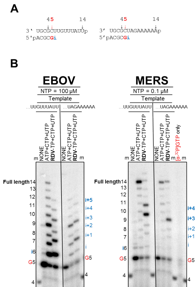
Figure 2. Patterns of inhibition of RNA synthesis with remdesivir-TP (RDV-TP). (A) RNA primer/template substrates used to test multiple (left) or single (right) incorporations of RDV-TP. G indicates incorporation of the radiolabeled nucleotide opposite template position 5. i indicates incorporation site for the first (left) or the only (right) RDV-TP. Full length indicates the full-template length products of RNA synthesis. (B) RDV-TP incorporation was monitored with purified EBOV and MERS RdRp complexes in the presence of indicated combinations of NTPs and RDV-TP.
