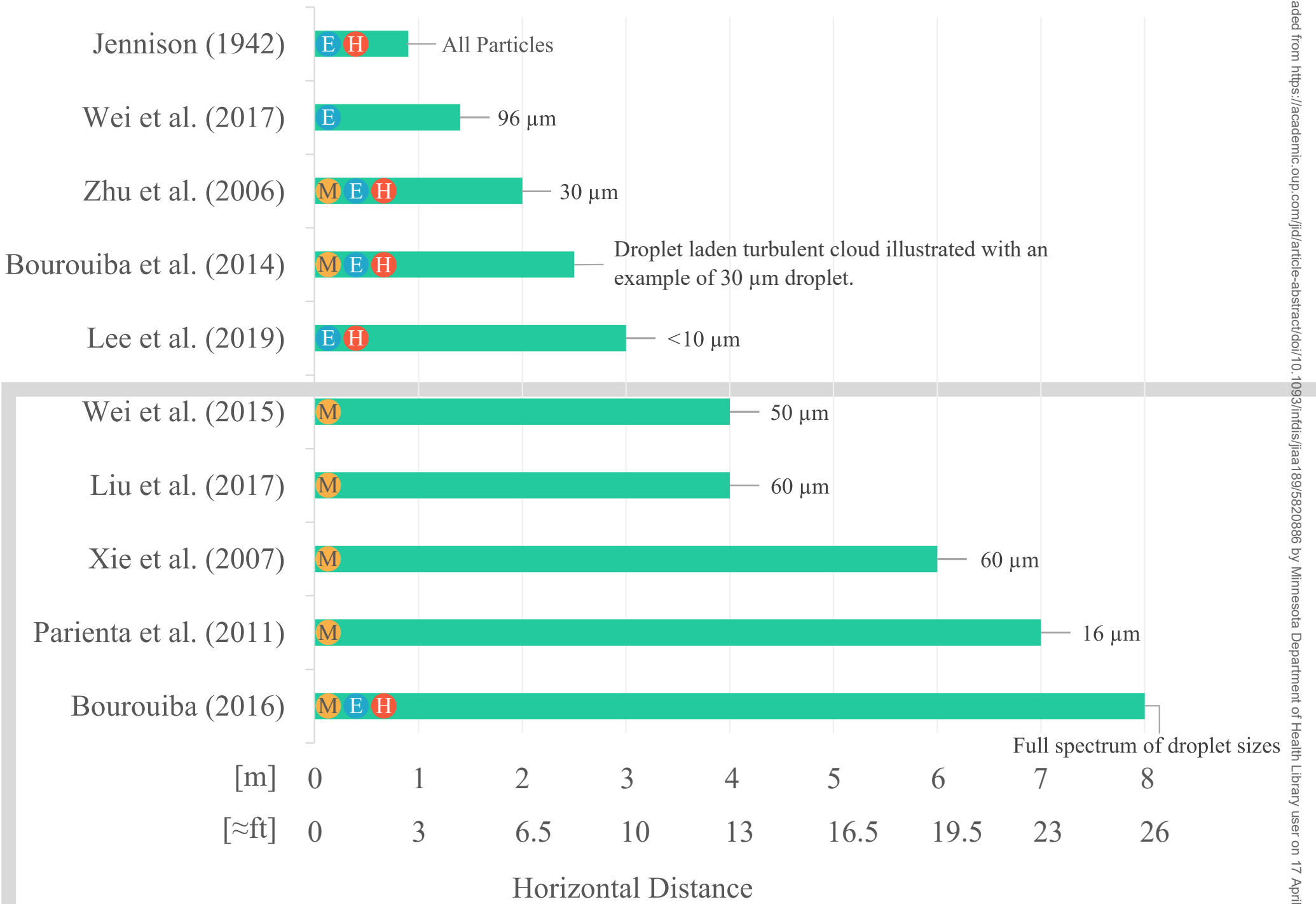
Figure 2: Extent of horizontal spread of droplets. M: Modelling (mathematical or numerical) studies; E: Experimental studies; H: Human subjects
