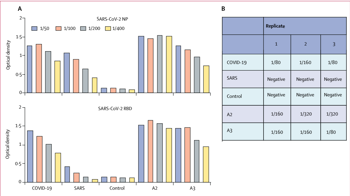
Figure 3: Serological testing of two patients (A) ELISA testing using SARS-CoV-2 NP and RBD antigens. In addition to serum samples from the two suspected cases (A2 and A3), known positive samples for COVID-19 and SARS, and negative samples, were included in the testing, and serial dilutions were done. (B) VNT results at the highest dilution that could effectively neutralise the SARS-CoV-2 infection. COVID-19=coronavirus disease 2019. NP=nucleocapsid protein. RBD=receptor binding domain. SARS=severe acute respiratory syndrome. SARS-CoV-2=severe acute respiratory syndrome coronavirus 2. VNT=virus neutralisation test.
