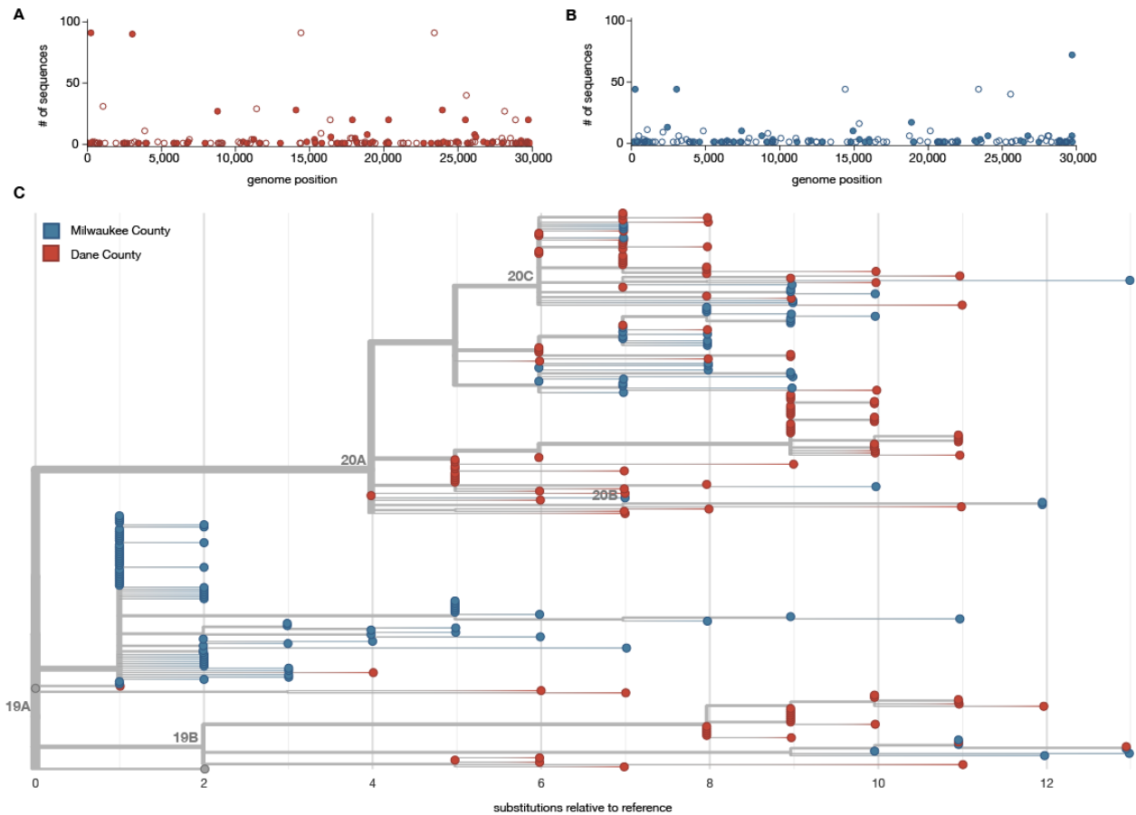
Figure 2. Characterizing consensus-level variants and sequence divergence among Dane and Milwaukee County sequences. SNVs are annotated relative to the initial Wuhan SARS-CoV-2 reference (Genbank: MN908947.3). A) Frequency of consensus SNVs among the Dane County sequences. B) Frequency of consensus SNVs among the Milwaukee County sequences. Open symbols denote synonymous or intergenic SNVs and closed symbols denote nonsynonymous SNVs. C) A divergence-based phylogenetic tree built using Nextstrain tools for the 122 Dane County (red) and 125 Milwaukee County (blue) sequences. Wisconsin samples are rooted against Wuhan-Hu-1/2019 and Wuhan/WH01/2019.
