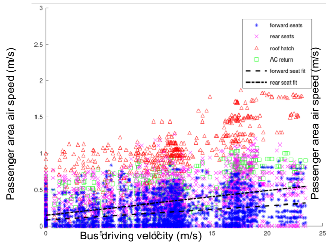
A. All windows half open, roof hatch
