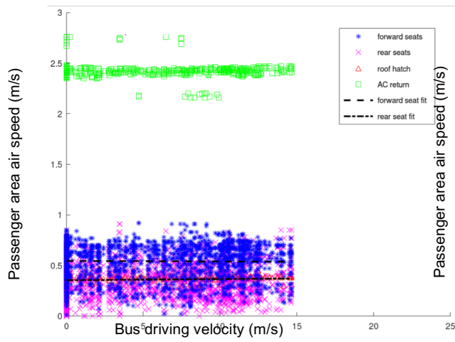
C. AC system with all windows closed
