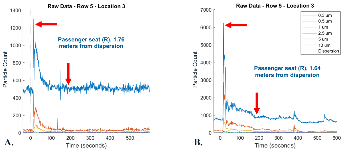
Figure S9: Particle count time-series waveforms on the school bus (A) and transit bus (B) showing the effects from the inclement weather configurations with a slightly widened peak (upper arrow) and slightly elongated residence time of particles (lower arrow) compared to all windows open.
