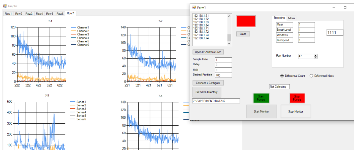
Figure S6: Screenshot of the custom multitreaded supervisory control and data acquisition (SCADA) software for nanoparticle dispersion test equipment
