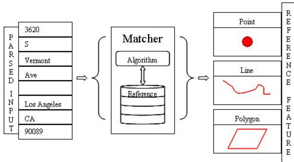
Figure 13 – Generalized feature-matching algorithm
