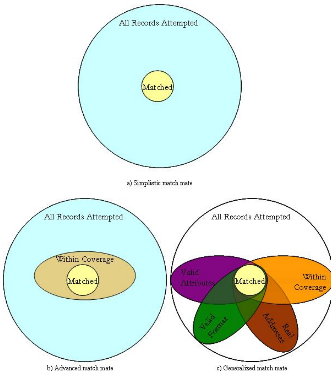
Figure 23 – Match rate diagrams
