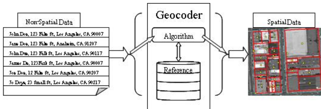
Figure 3 - Schematic showing basic components of the geocoding process
