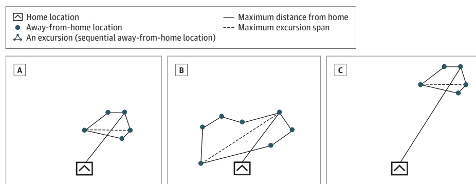
Figure 1. Schematic of Distance-Based Metrics
