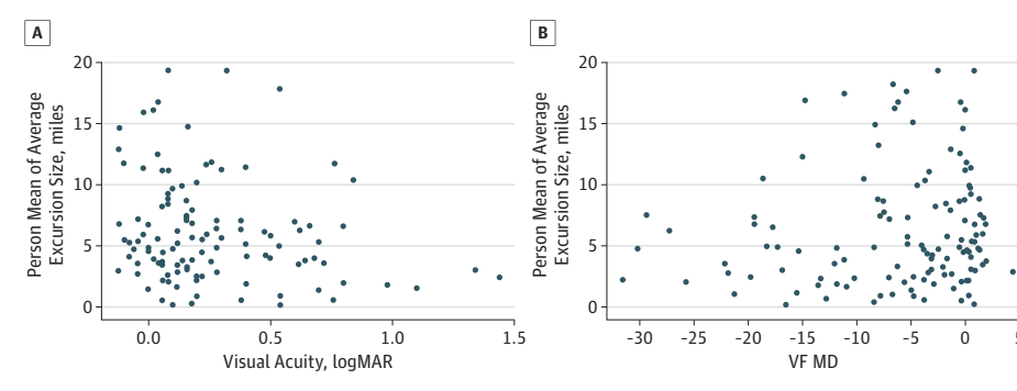
Figure 2. Scatterplots of Daily Average Excursion Size
